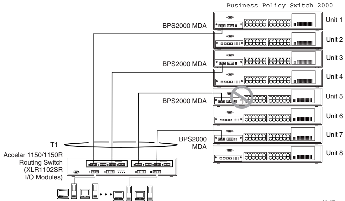
Figure 42 Loss of distributed trunk members
