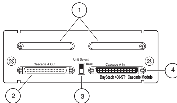
Figure 12 BayStack 400-ST1 Cascade Module front-panel components
