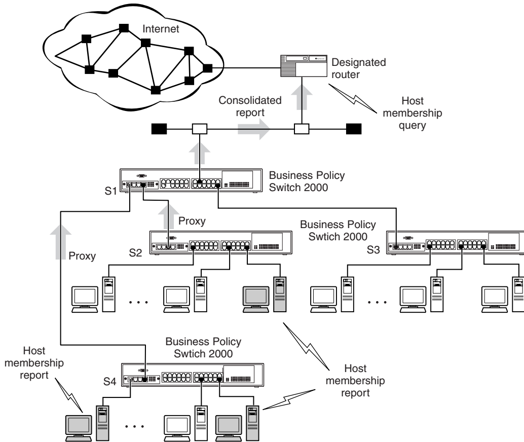
Figure 36 Business Policy Switch filtering IP multicast streams (1 of 2)
